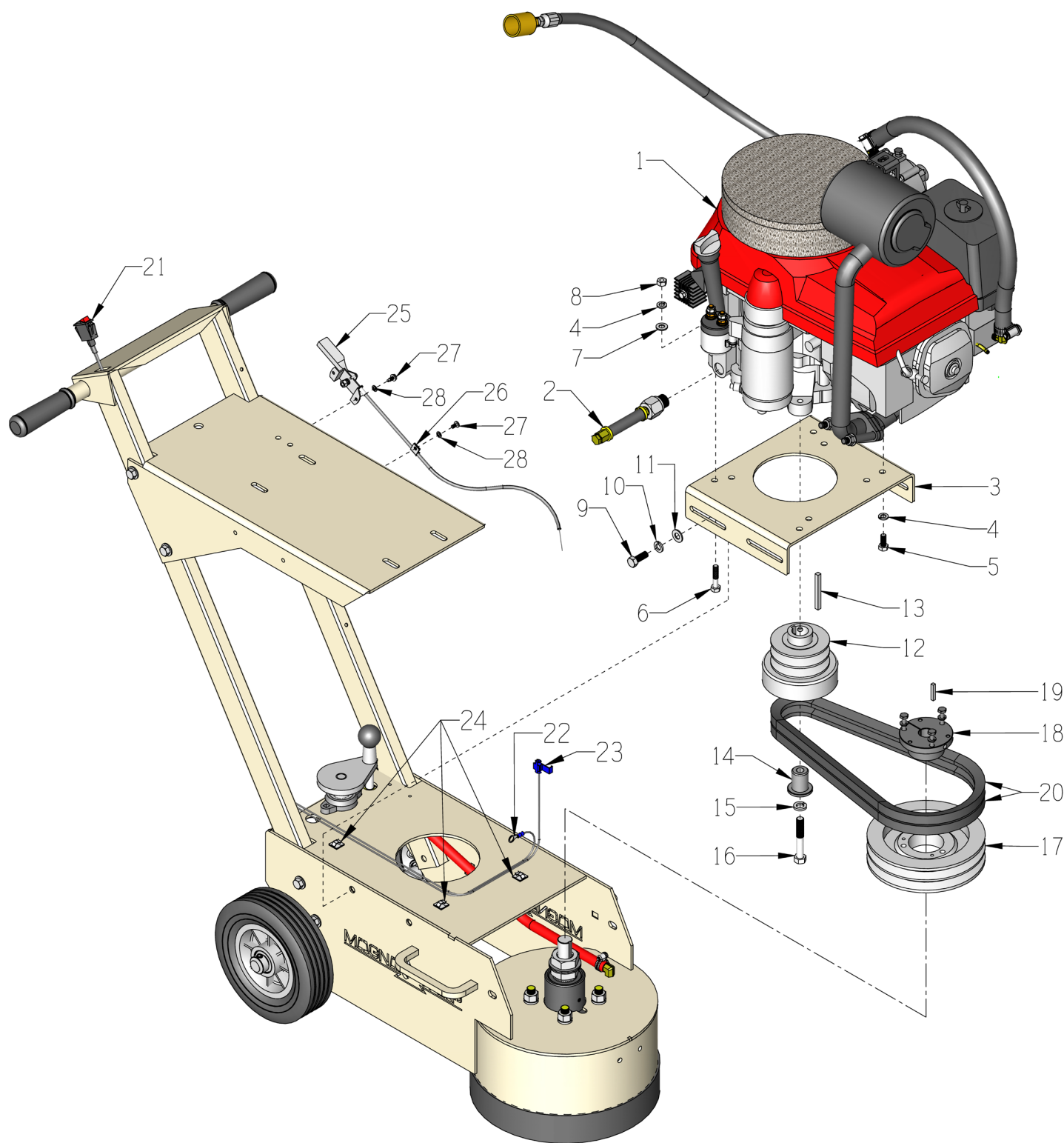
ILLUSTRATION 11: PROPANE ENGINE & BELT DRIVE GROUPING
