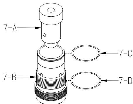
ITEM # 7 PART # 27028 PISTON & CYLINDER ASSEMBLY
