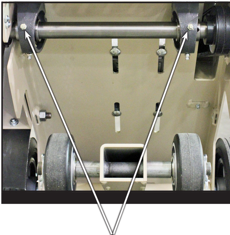
Grease Fittings
